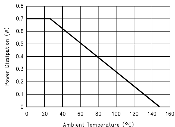
LM4900LD Power Derating Curve (Note 12)
